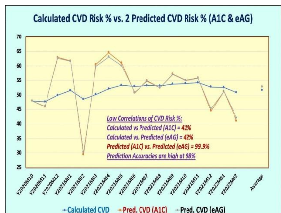
Figure 5: 2 Predicted CVD risk % versus calculated CVD risk % using visco-perturbation model.
