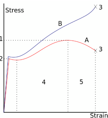
A stress-strain is typical of structural steel.
