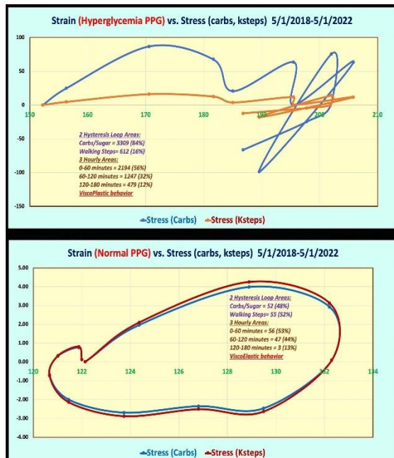
Figure 2: Stress-strain diagram of both Hi-PPG & normal PPG based on the VGT energy model with two risk factors (carbs and steps).
