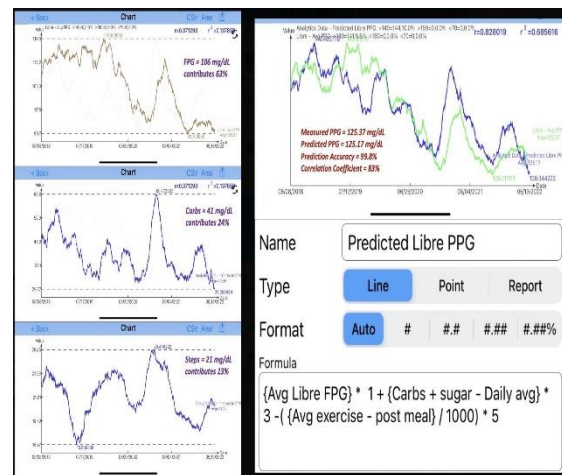
Figure 1: Time-domain analysis of FPG, diet, exercise, and LGT predicted PPG.
