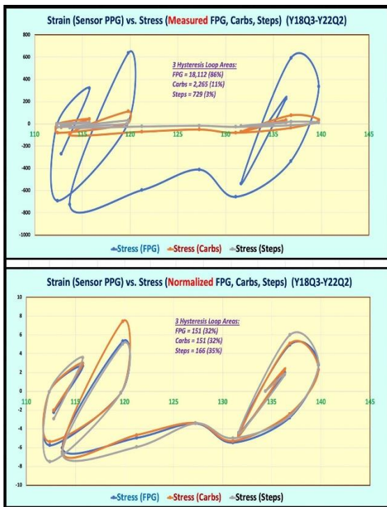
Figure 3: 2 VGT stress-strain diagrams & hysteresis loop areas.
