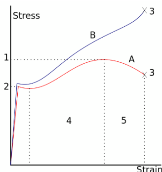
A stress-strain is typical of structural steel.
