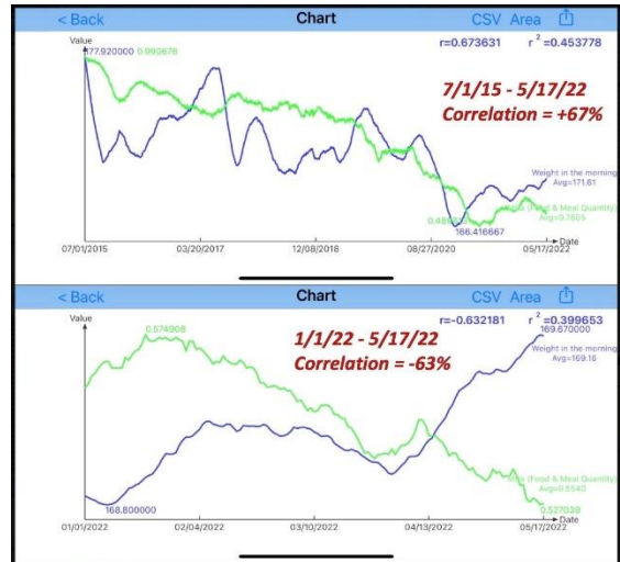
Figure 3: Correlation coefficients analyses for different time windows (long vs. short).
