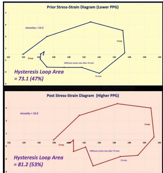
Figure 5: 2 VGT stress-strain diagrams & hysteresis loop areas for hyper-PPG study.
