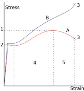
A stress-strain is typical of structural steel.
