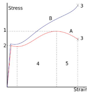
A stress-strain is typical of structural steel.
