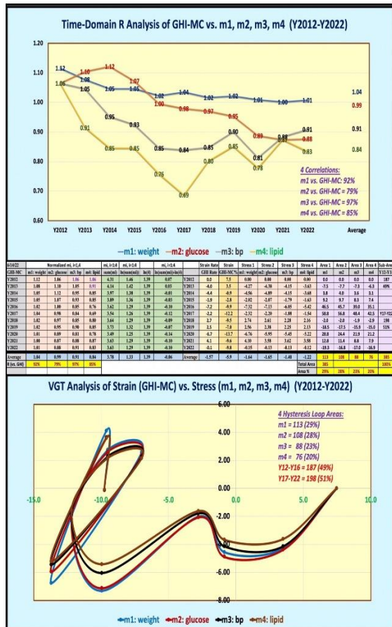
Figure 1: TD-correlation analysis, SD-VGT analysis results of GHI-MC with a data table.
