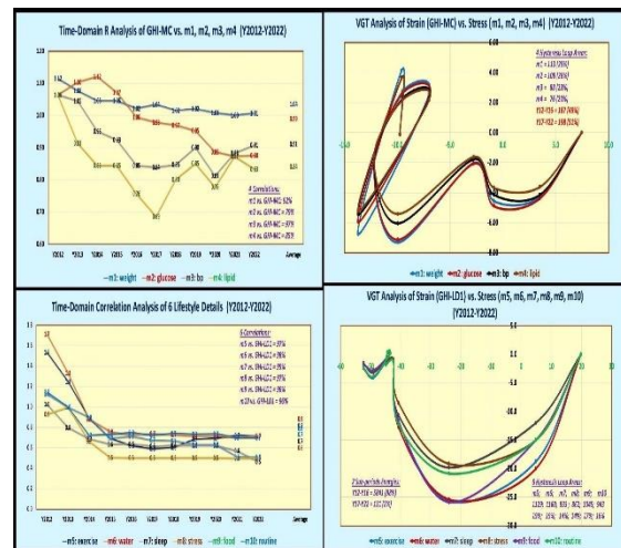
Figure 3: Comparison of both TD results and SD results of MC and LD.
