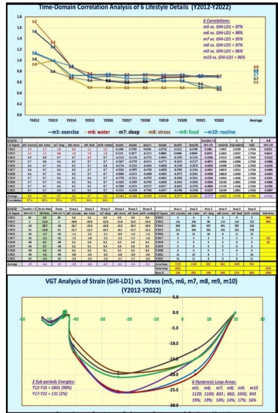
Figure 2: TD-correlation analysis, SD-VGT analysis results of GHI-LD with a data table.
