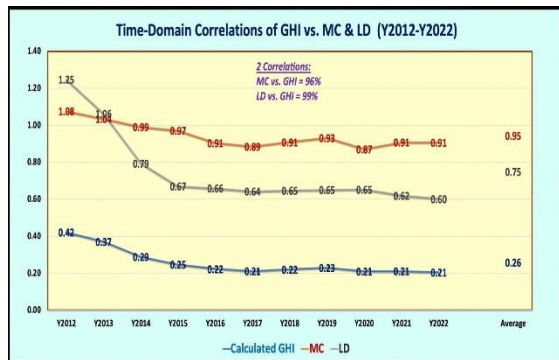
Figure 1: TD-correlation analysis results.
