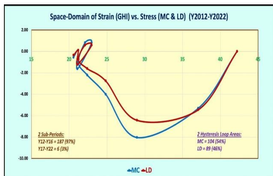
Figure 2: SD-VGT analysis results of GHI vs. MC no LD.
