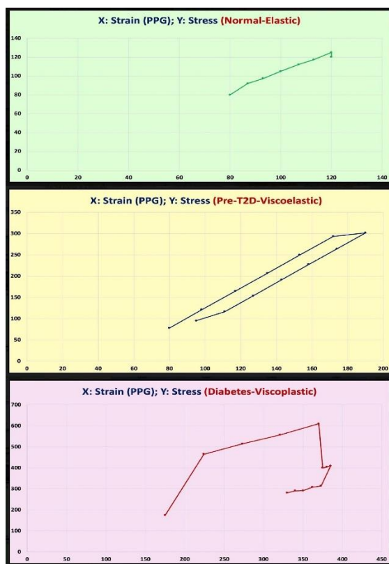
Figure 3: Stress-strain diagrams of 3 standard cases.
