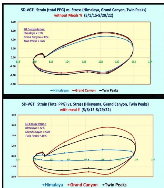
Figure 3: 2 SD-VGT viscoelastic stress-strain diagrams.
